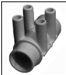
X272700 1-1/2" SxSpg x 3/4" 4 Barb Manifold
