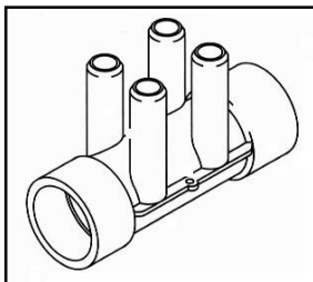
X272600 1-1/2" SxS x 3/4" 4 Barb Manifold
