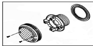
X250622 2" Suction Wallfitting X250623 Gasket
