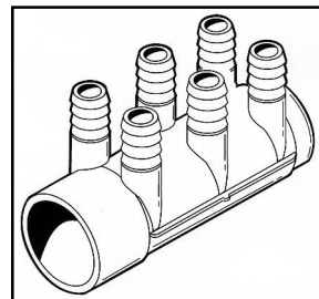
X272920 2" x 3/4" SxS 6 Barb Manifold
