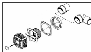
X250050 200 GPM 90 degree Suction ~ Grey
